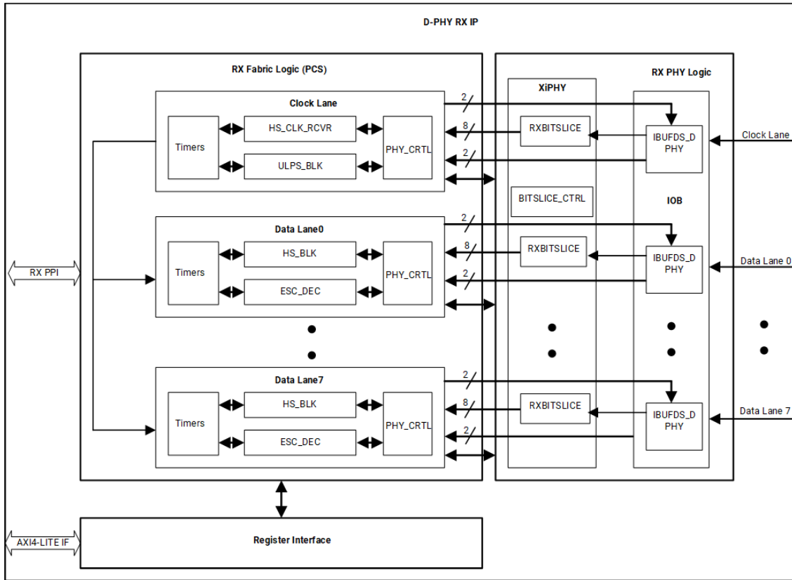
Figure 18: MIPI D-PHY RX Architecture
