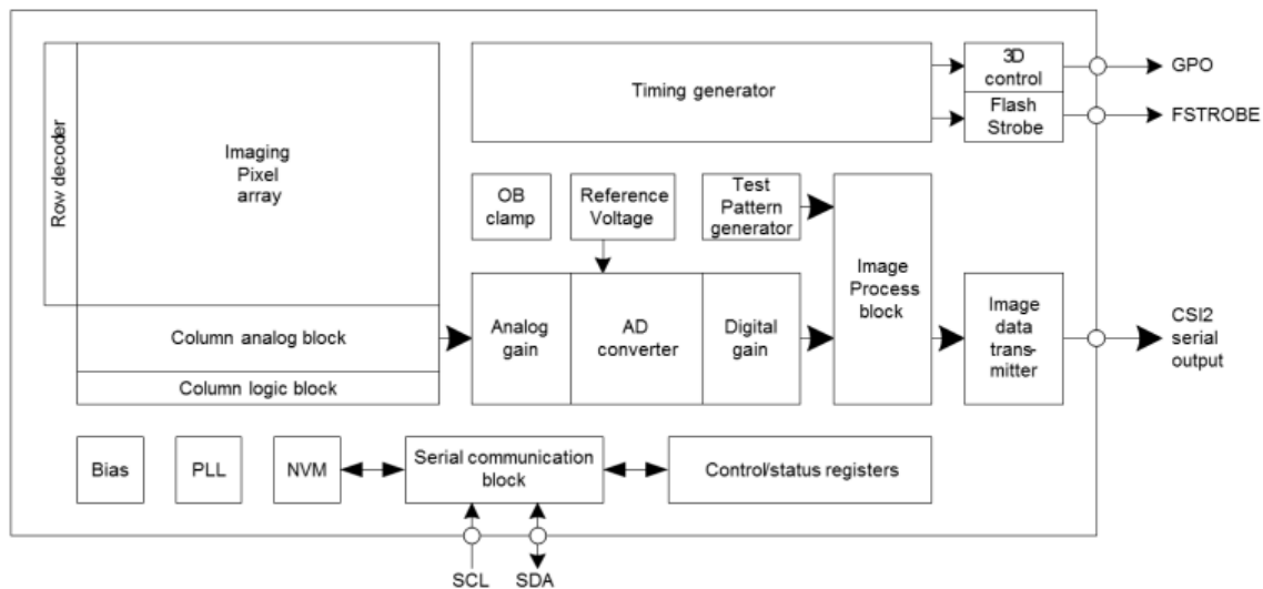
Figure 11: IMX219 Block Diagram
