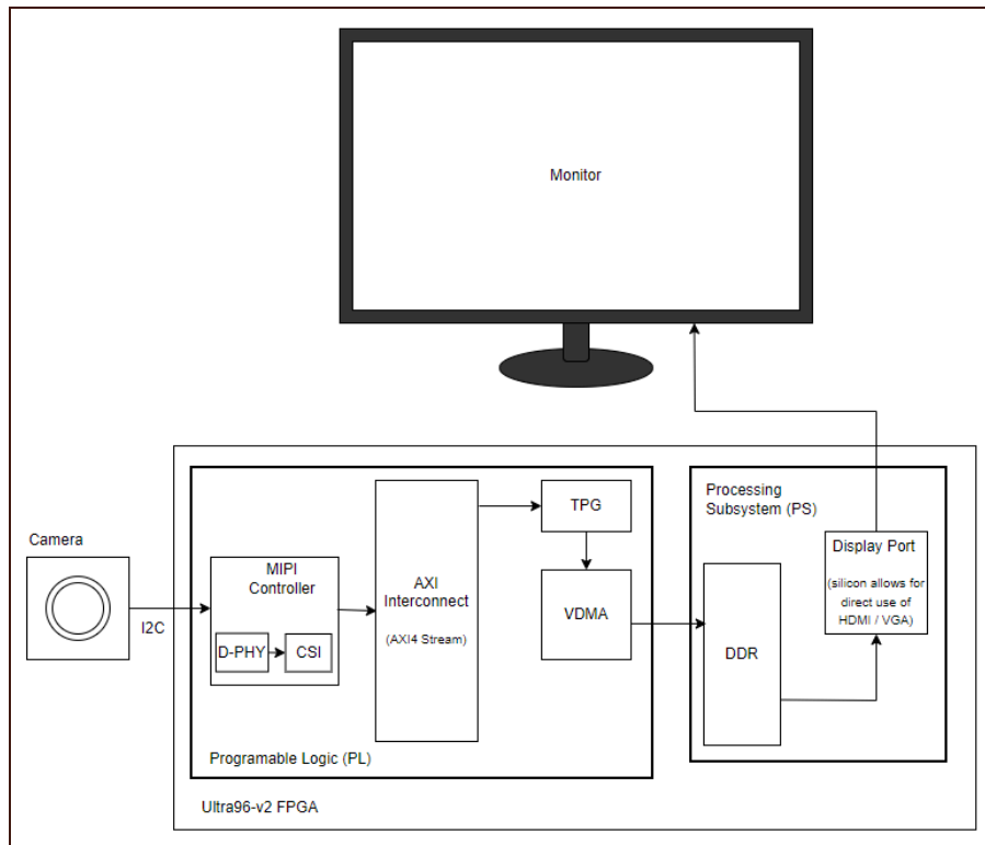
Figure 22: Datapath for the Video Stream
