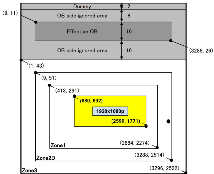
Figure 14: The Frame Structure for 1920x1080p
