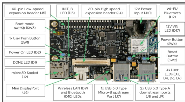
Figure 8: Anatomy of Ultra-96 FPGA
