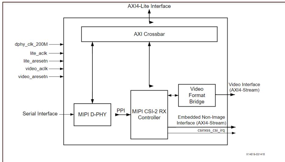
Figure 17: MIPI Subsystem Block Diagram
