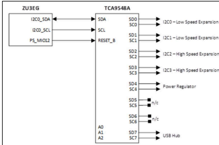
Figure 15: I2C Block Diagram
