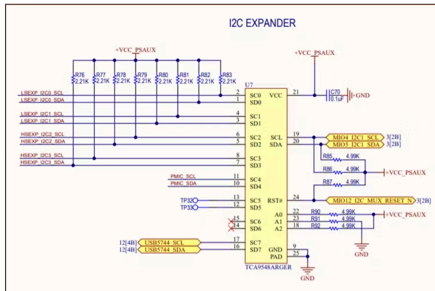
Figure 16: I2C Expander
