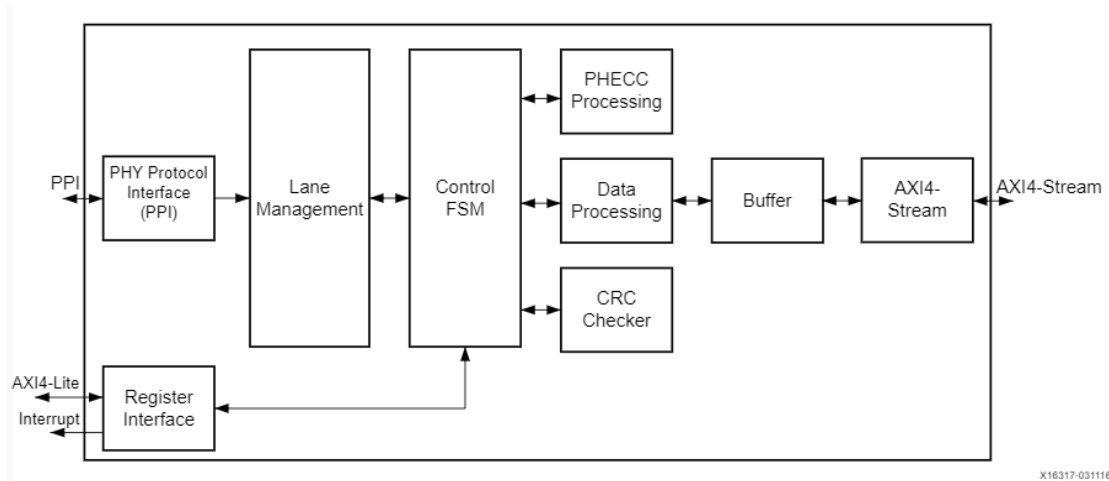
Figure 19: MIPI CSI-2 RX Architecture
