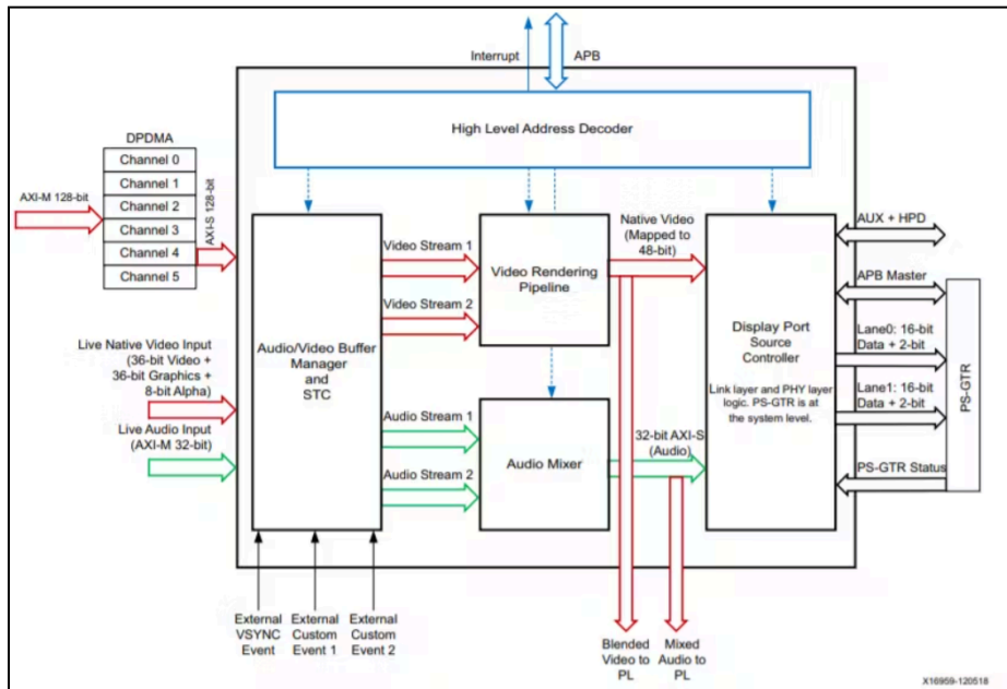
Figure 21: Ultra96-v2 Displayport Controller Architecture
